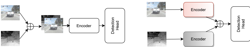
Figure 7: Schematic diagram of the Input Fusion and Feature Fusion methods respectively. (a) Input Fusion - combines RGB and thermal into a new dataset and trains the network (b) Feature Fusion - concatenates features from RGB and Thermal Encoders and trains the detection head
