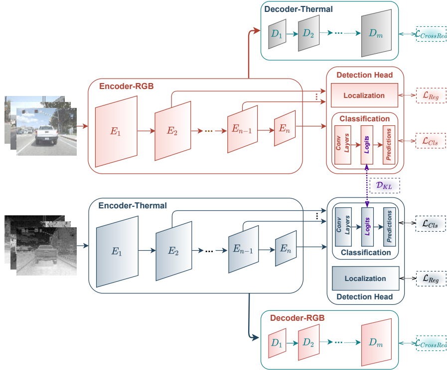
Figure 6: Schematic diagram of the MultiModal-Collaborative Learning framework with Cross Reconstruction. The encoder is DeiT-Tiny and SSD is the detection head. In MMC+Cross Reconstruction variant, the intermediate features of the RGB image (i.e, features from RGB encoder) are passed to the thermal decoder to reconstruct the original RGB image and vice-versa. The networks are trained with a supervised classification ( \mathcal{L}_{Cls} ) and regression loss ( \mathcal{L}_{Reg} ), a mimicry loss ( D_{KL} ) and an auxiliary cross reconstruction loss ( \mathcal{L}_{CrossRec} ).
