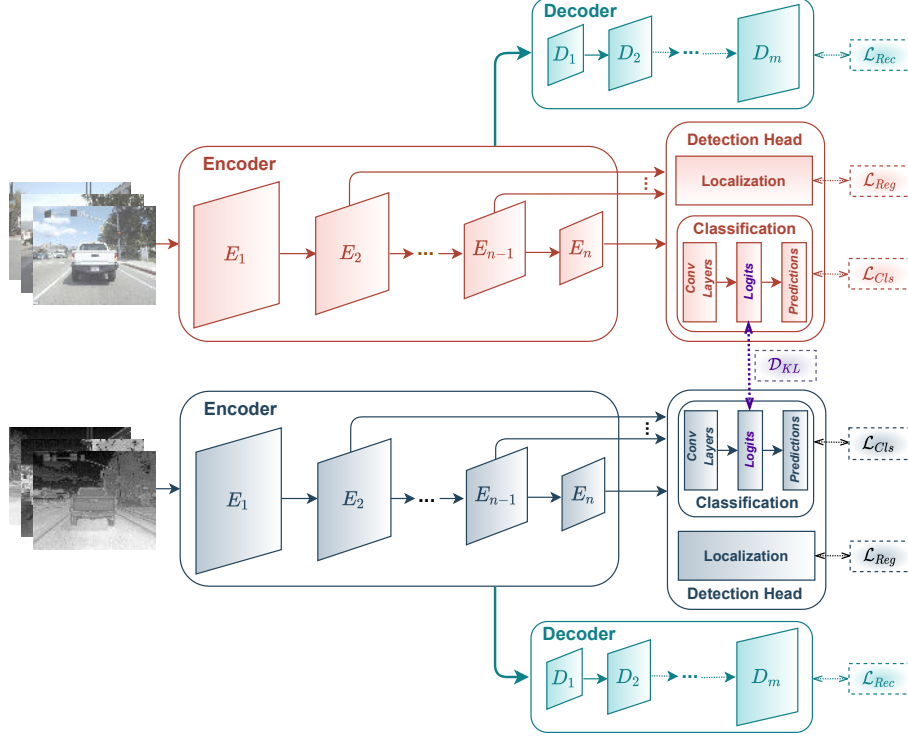
Figure 2: Schematic diagram of the MultiModal-Collaborative Learning framework. The encoder is DeiT-Tiny and SSD is the detection head. The network with red hue represents the RGB-network and the network with grey hue represents the thermal-network. The networks are trained with a supervised classification ( \mathcal{L}_{Cls} ) and regression loss ( \mathcal{L}_{Reg} ), a mimicry loss ( D_{KL} ) and an auxiliary reconstruction loss ( \mathcal{L}_{Rec} ).
