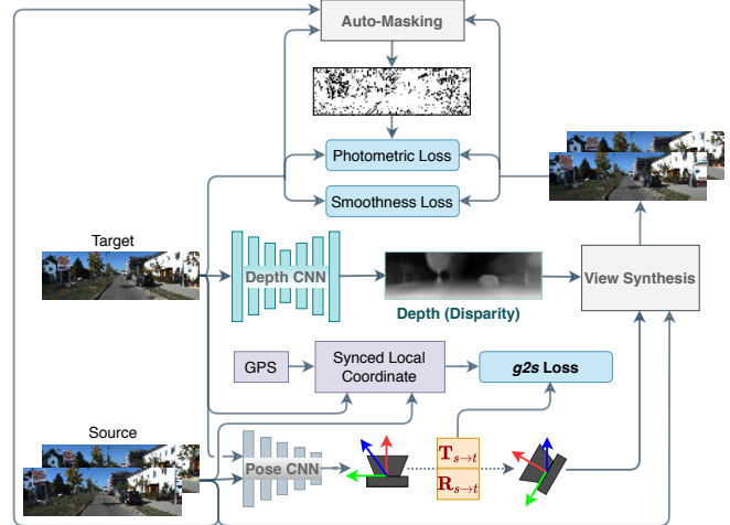
Fig. 1. A schematic of our proposed multimodal self-supervised depth and ego-motion prediction network for monocular videos. We introduce a GPS-to-Scale ( g2s ) loss that leads to scale-consistent and -aware estimates during inference.
