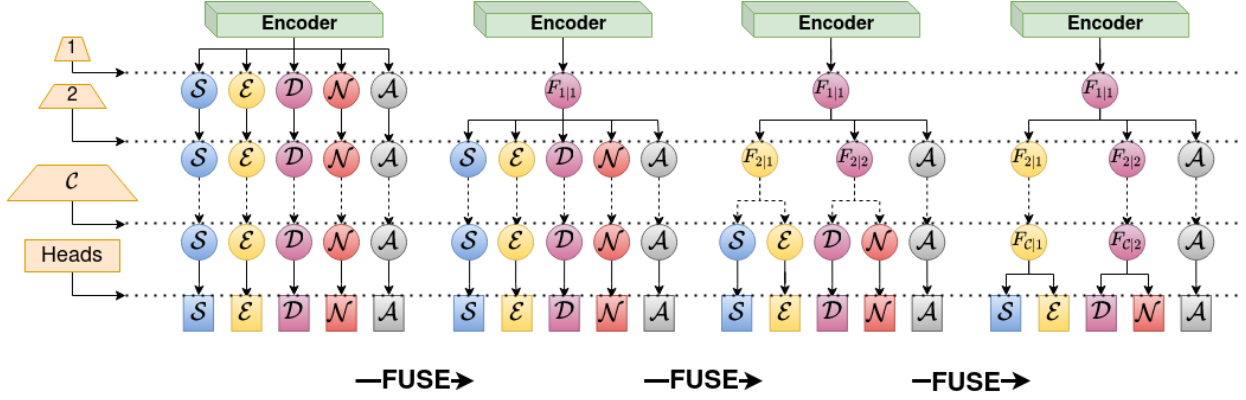
Figure 1: Fusing decoders at different candidate stages. From left to right decoder fusion at candidate stages 1, 2 and C is shown. S, E, D, N and A denote different tasks, namely semantic segmentation, edge detection, depth estimation, surface normals and autoencoder. The dotted horizontal lines show the candidate decoder stages and the task-specific heads. The lines connecting decoder stages in 2 and C are dotted to show that there are more stages in between. The task-specific heads are not fused in any of the approaches. \mathcal{F} denotes fused decoder and \mathcal{F}_{i|j} denotes i^{th} candidate stage of j^{th} task decoder.
